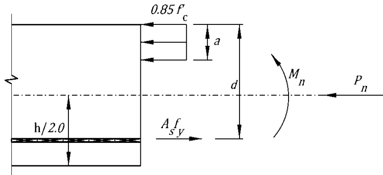
Figure D-1. Section of Stress for Singly Reinforced Member.
